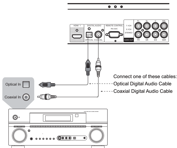
Receiver/Amplifier with Dolby Digital or DTS Decoder
