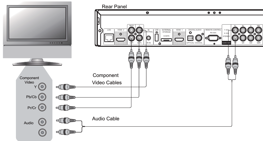
Method 3 – Component Video Connection to TV
