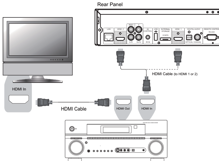
Method 4 – HDMI Connection to Receiver and TV
